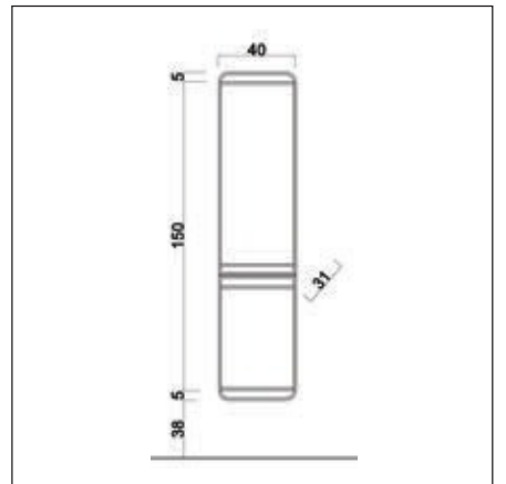
TALL CABINET
